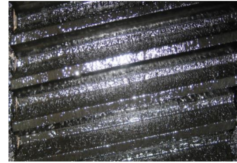
Actual appearance of Drag Drum Open Gear lubricated with Molub-Alloy OG 968 SF Heavy
